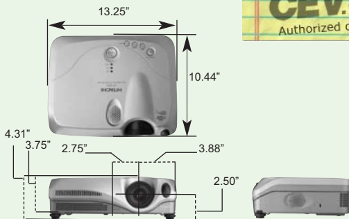
CP-X445 Dimensions (Incl. protruding part)
